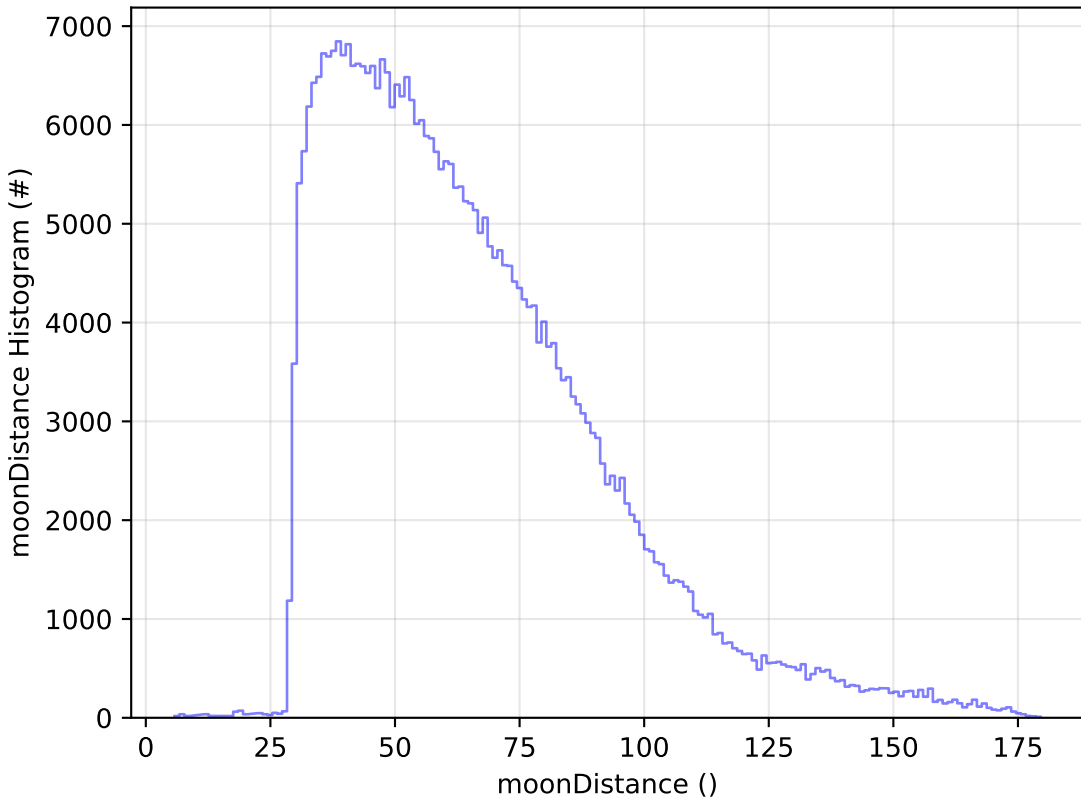
too_5_4v3.4_10yrs WFD y band: moonDistance Histogram
