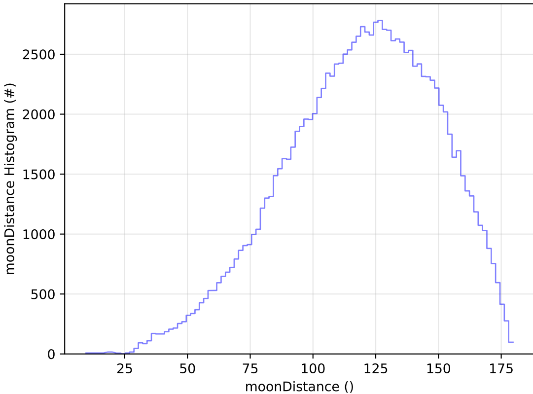
too_5_4v3.4_10yrs WFD u band: moonDistance Histogram
