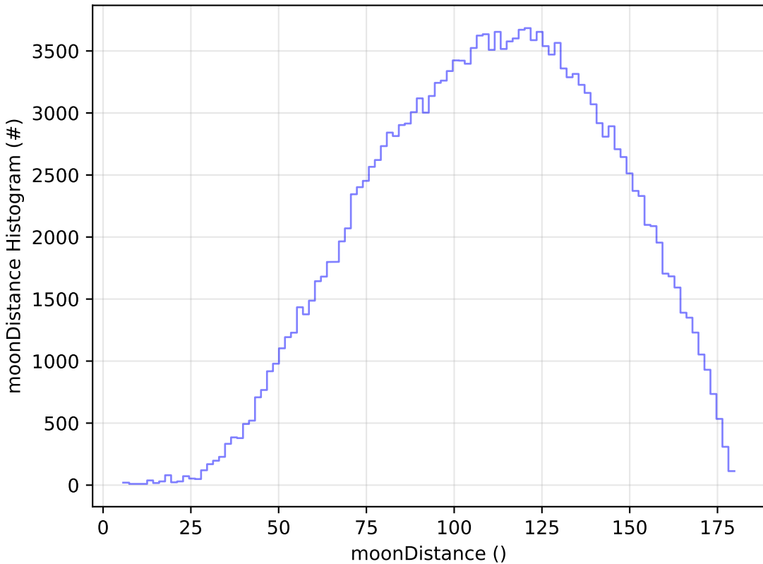
too_5_4v3.4_10yrs WFD g band: moonDistance Histogram
