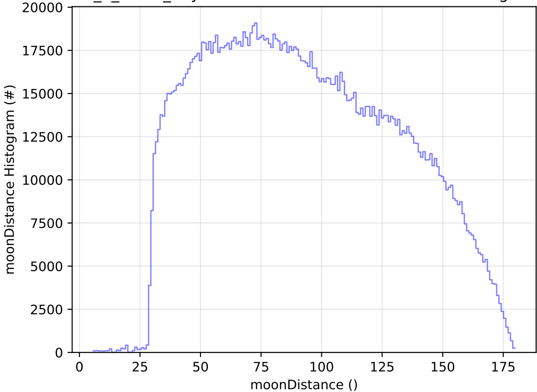
too_5_4v3.4_10yrs WFD all bands: moonDistance Histogram
