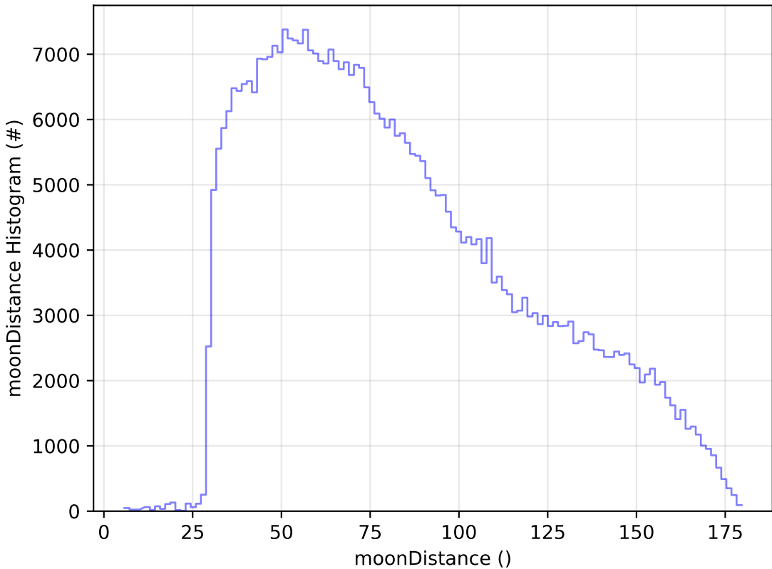
too_5_4v3.4_10yrs All sky z band: moonDistance Histogram
