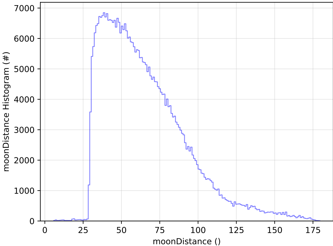
too_5_4v3.4_10yrs All sky y band: moonDistance Histogram
