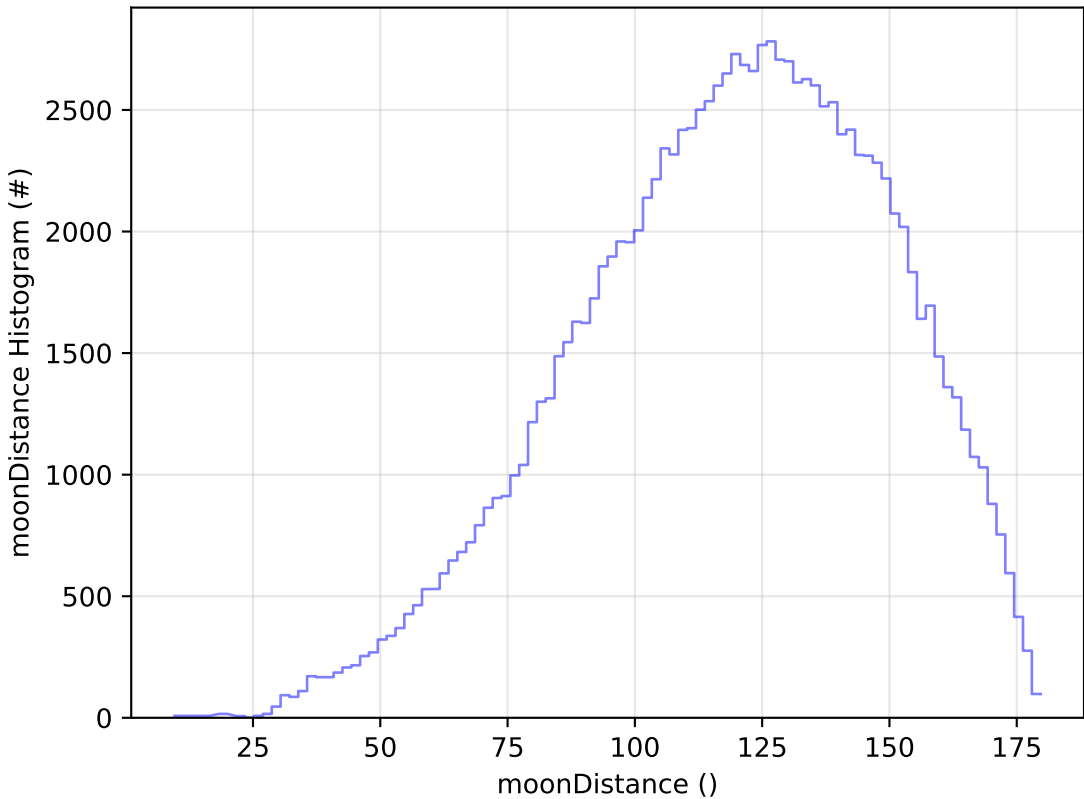
too_5_4v3.4_10yrs All sky u band: moonDistance Histogram
