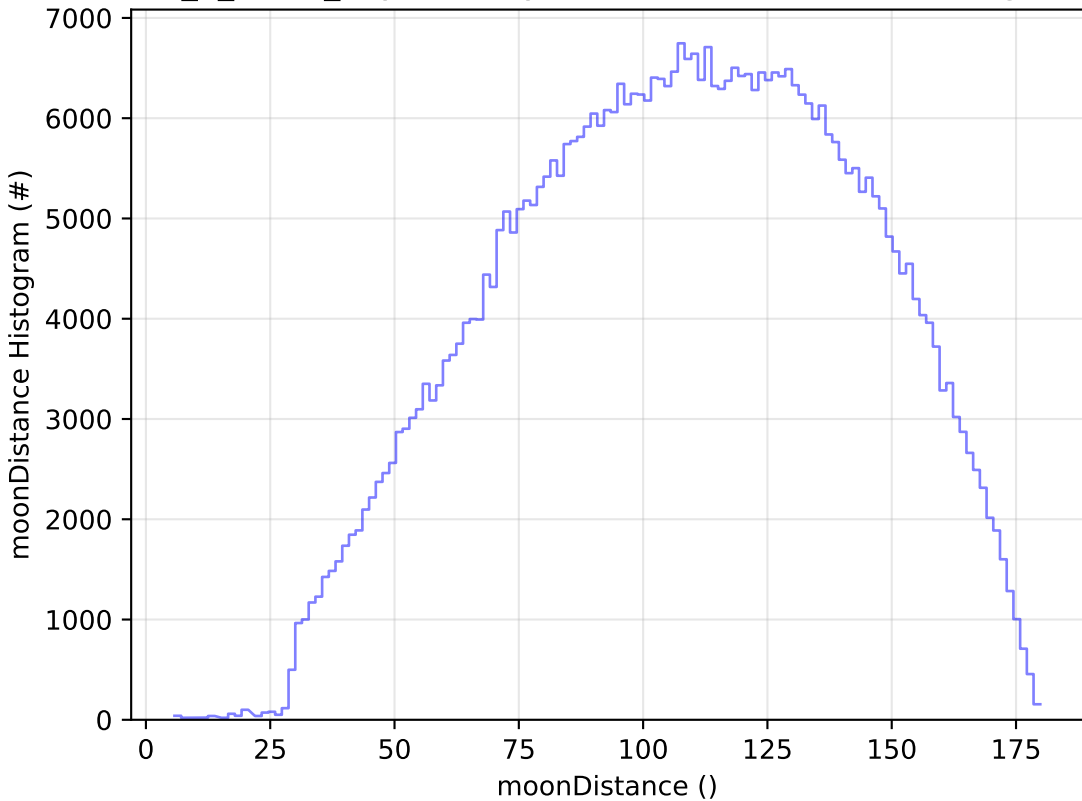
too_5_4v3.4_10yrs All sky r band: moonDistance Histogram
