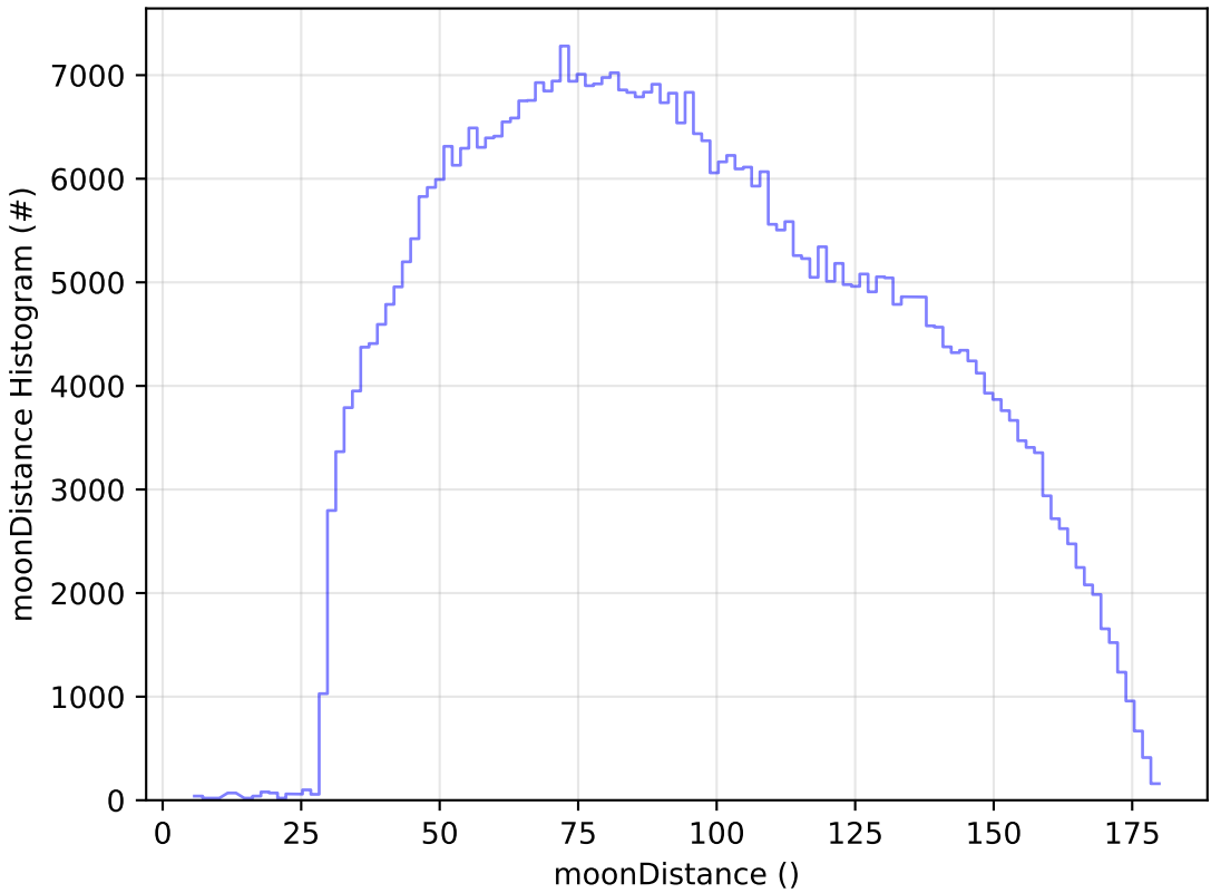
too_5_4v3.4_10yrs All sky i band: moonDistance Histogram
