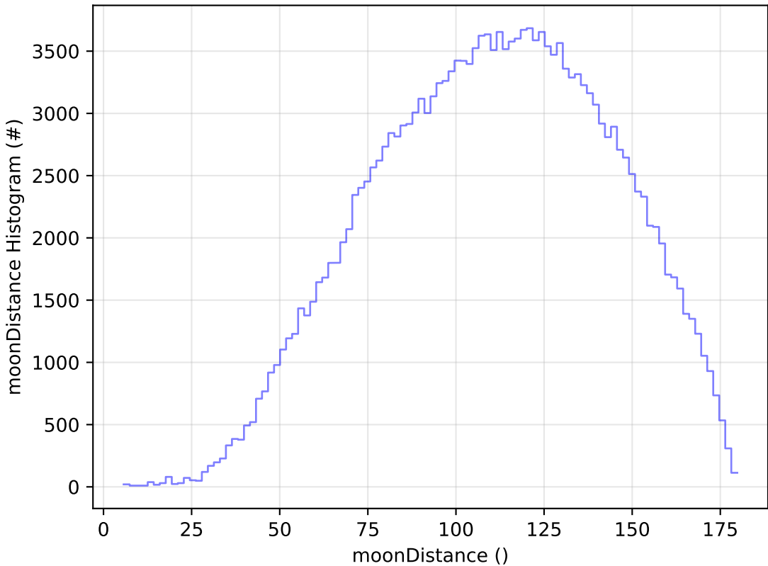
too_5_4v3.4_10yrs All sky g band: moonDistance Histogram
