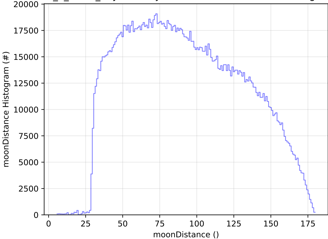
too_5_4v3.4_10yrs All sky all bands: moonDistance Histogram
