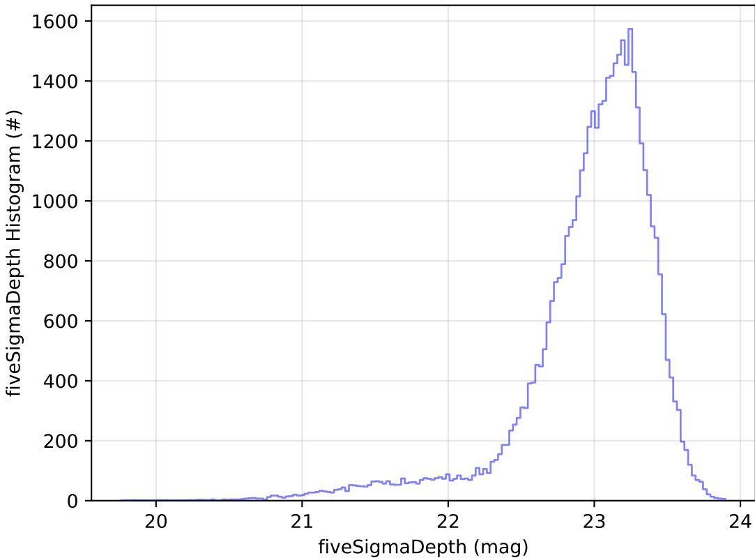
too_5_4v3.4_10yrs Yr 1 z band: fiveSigmaDepth Histogram
