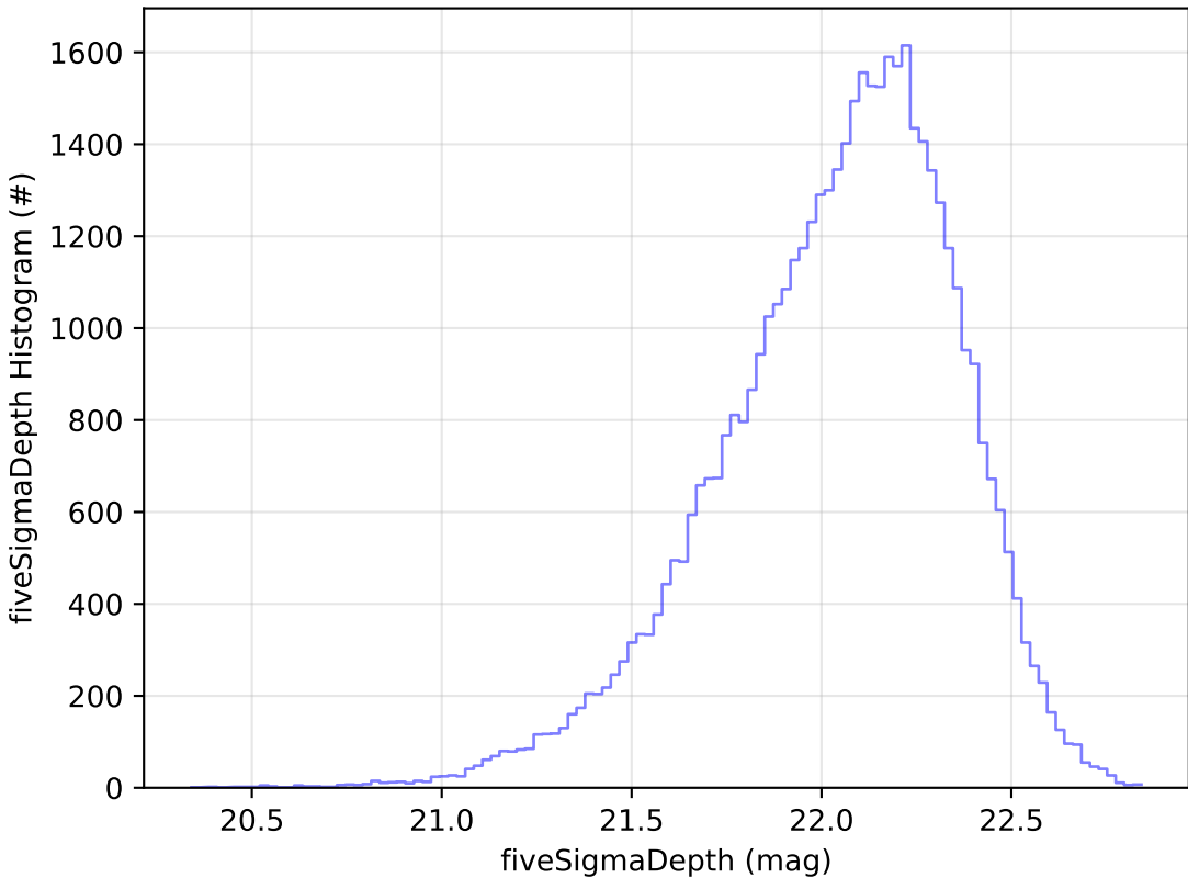
too_5_4v3.4_10yrs Yr 1 y band: fiveSigmaDepth Histogram
