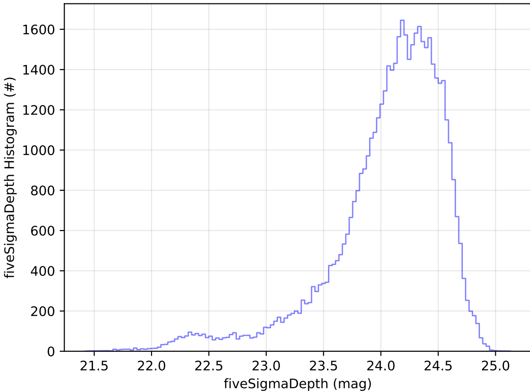
too_5_4v3.4_10yrs Yr 1 r band: fiveSigmaDepth Histogram
