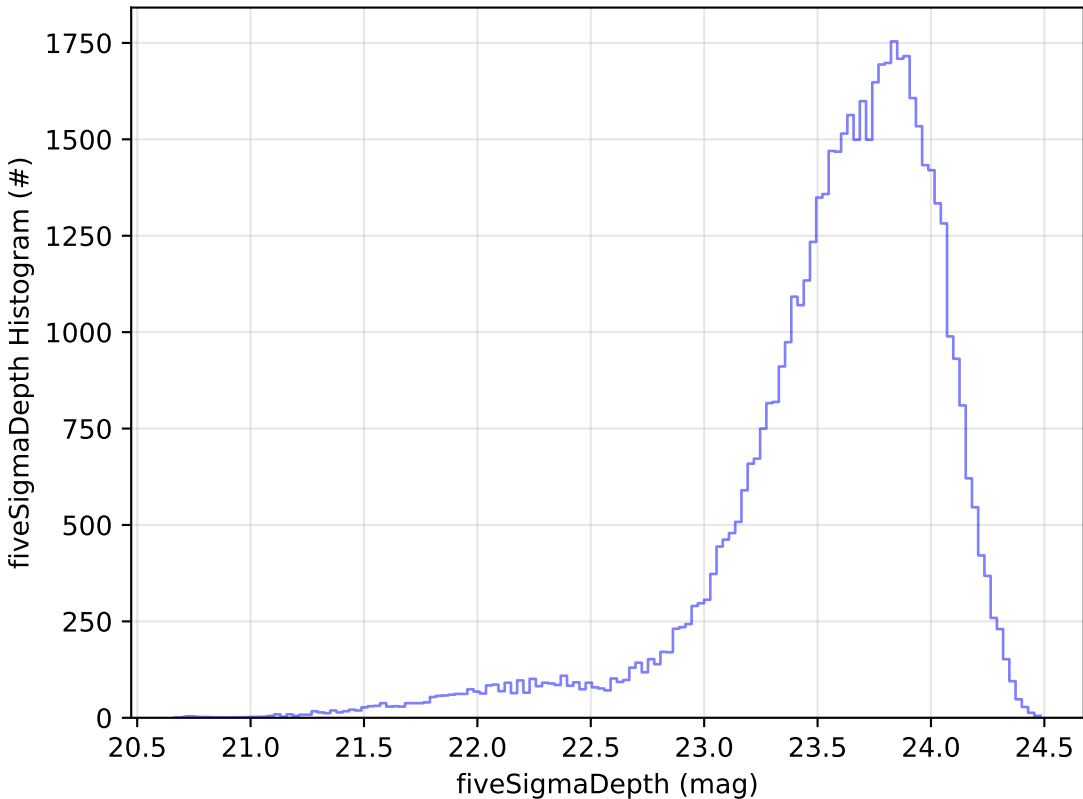
too_5_4v3.4_10yrs Yr 1 i band: fiveSigmaDepth Histogram
