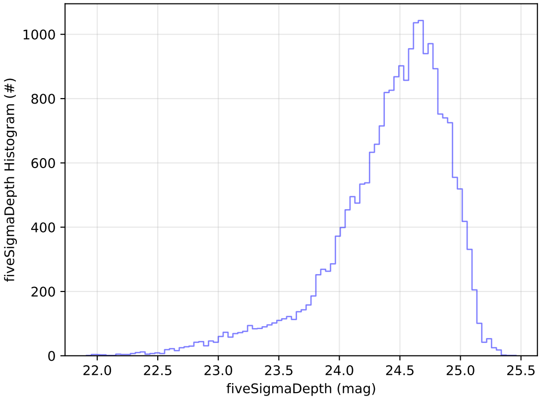
too_5_4v3.4_10yrs Yr 1 g band: fiveSigmaDepth Histogram
