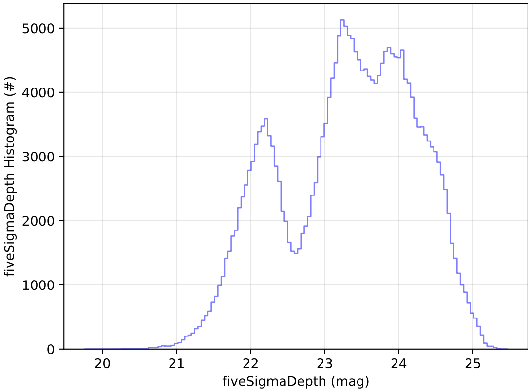
too_5_4v3.4_10yrs Yr 1 all bands: fiveSigmaDepth Histogram
