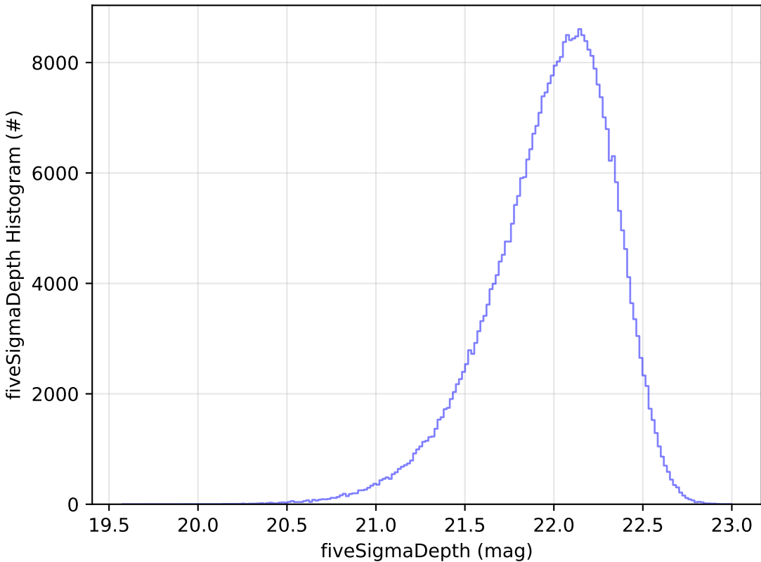
too_5_4v3.4_10yrs WFD y band: fiveSigmaDepth Histogram
