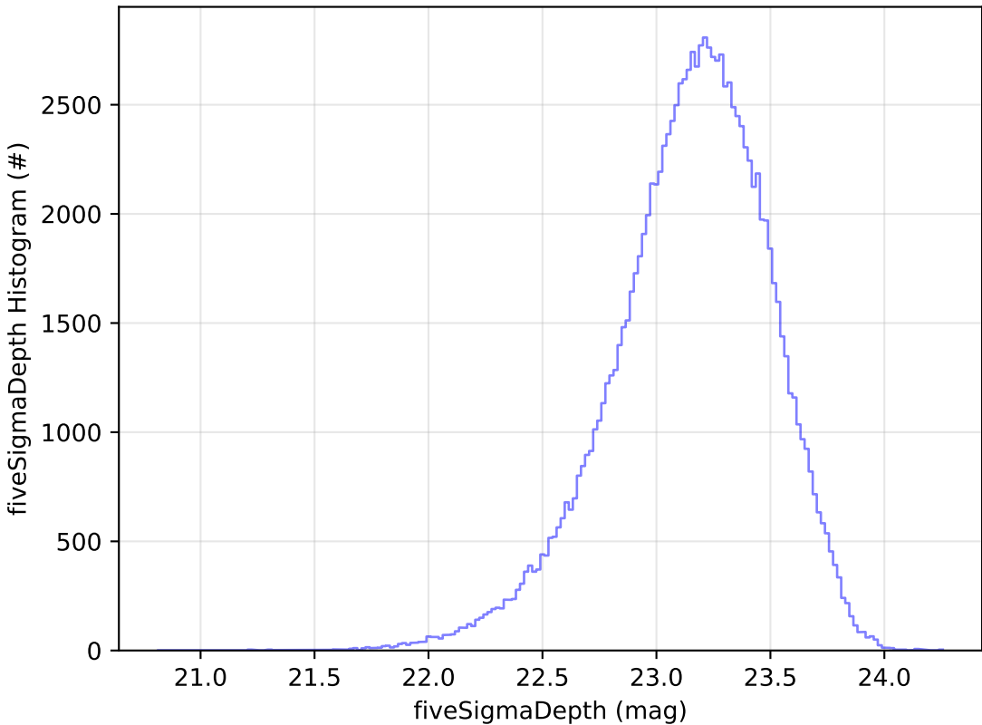
too_5_4v3.4_10yrs WFD u band: fiveSigmaDepth Histogram
