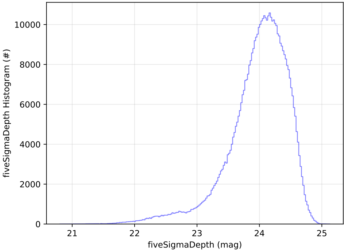
too_5_4v3.4_10yrs WFD r band: fiveSigmaDepth Histogram
