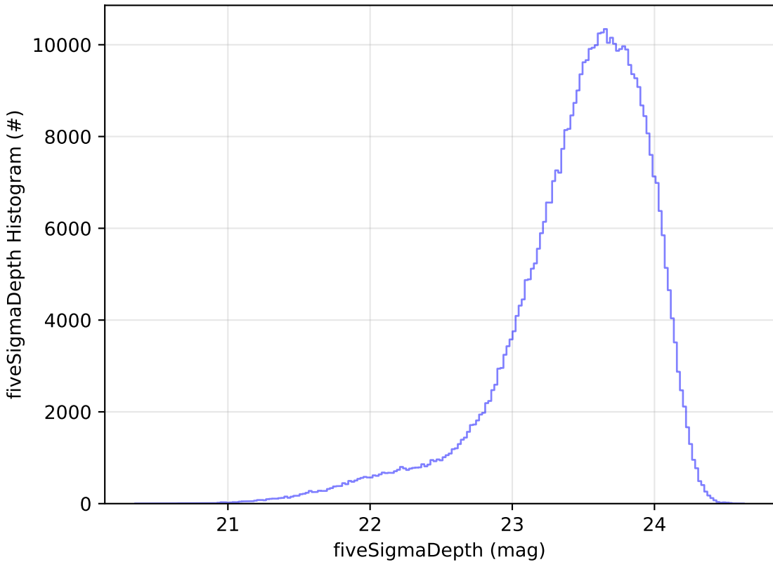
too_5_4v3.4_10yrs WFD i band: fiveSigmaDepth Histogram
