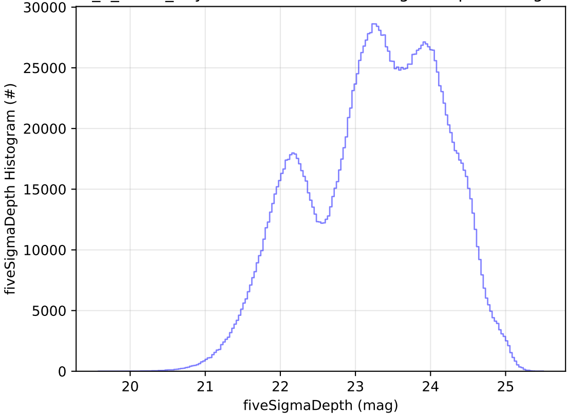
too_5_4v3.4_10yrs WFD all bands: fiveSigmaDepth Histogram
