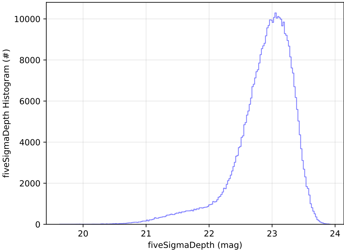
too_5_4v3.4_10yrs All sky z band: fiveSigmaDepth Histogram
