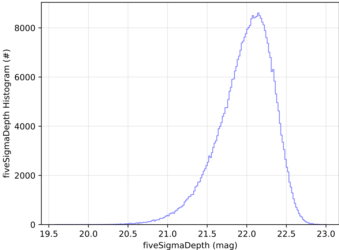
too_5_4v3.4_10yrs All sky y band: fiveSigmaDepth Histogram
