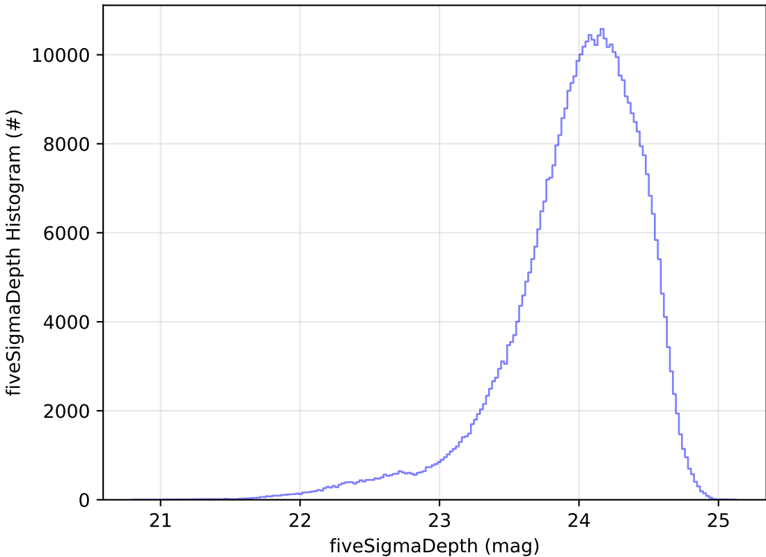
too_5_4v3.4_10yrs All sky r band: fiveSigmaDepth Histogram
