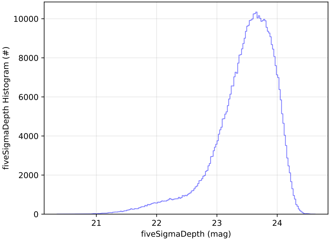
too_5_4v3.4_10yrs All sky i band: fiveSigmaDepth Histogram
