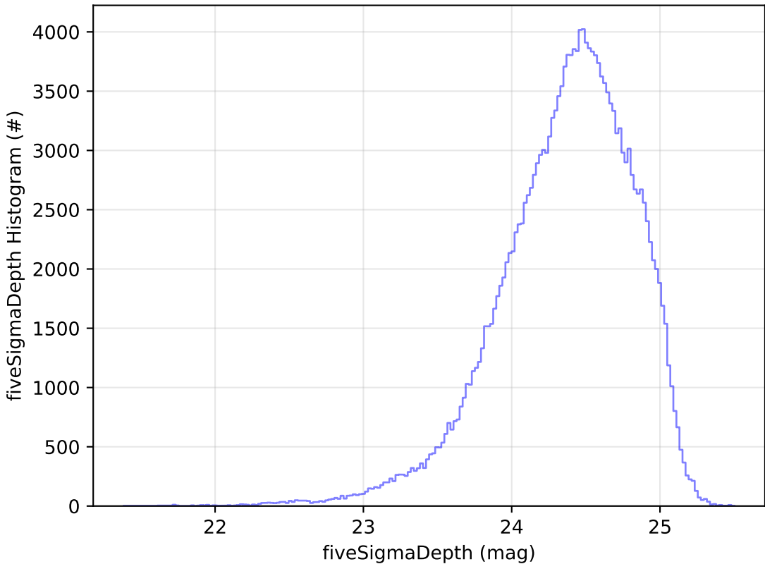
too_5_4v3.4_10yrs All sky g band: fiveSigmaDepth Histogram
