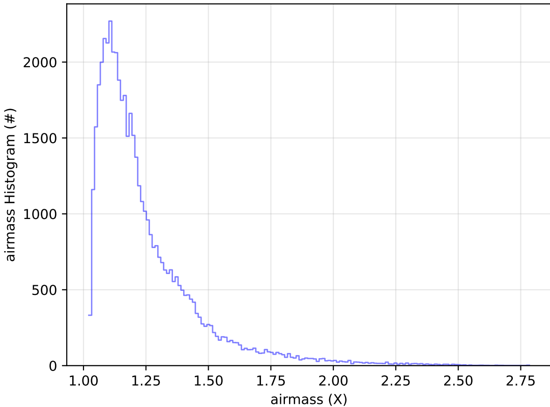
too_5_4v3.4_10yrs Yr 1 y band: airmass Histogram
