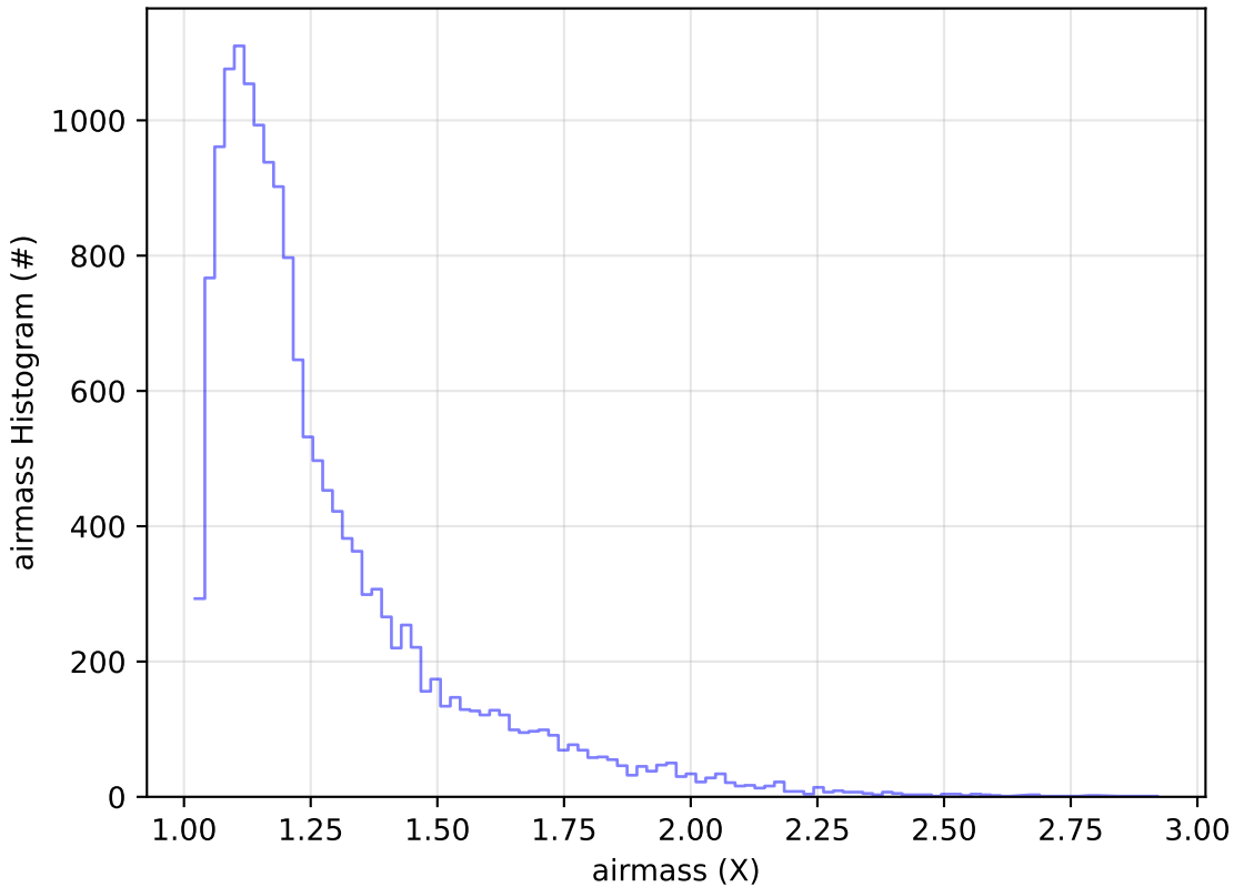
too_5_4v3.4_10yrs Yr 1 u band: airmass Histogram
