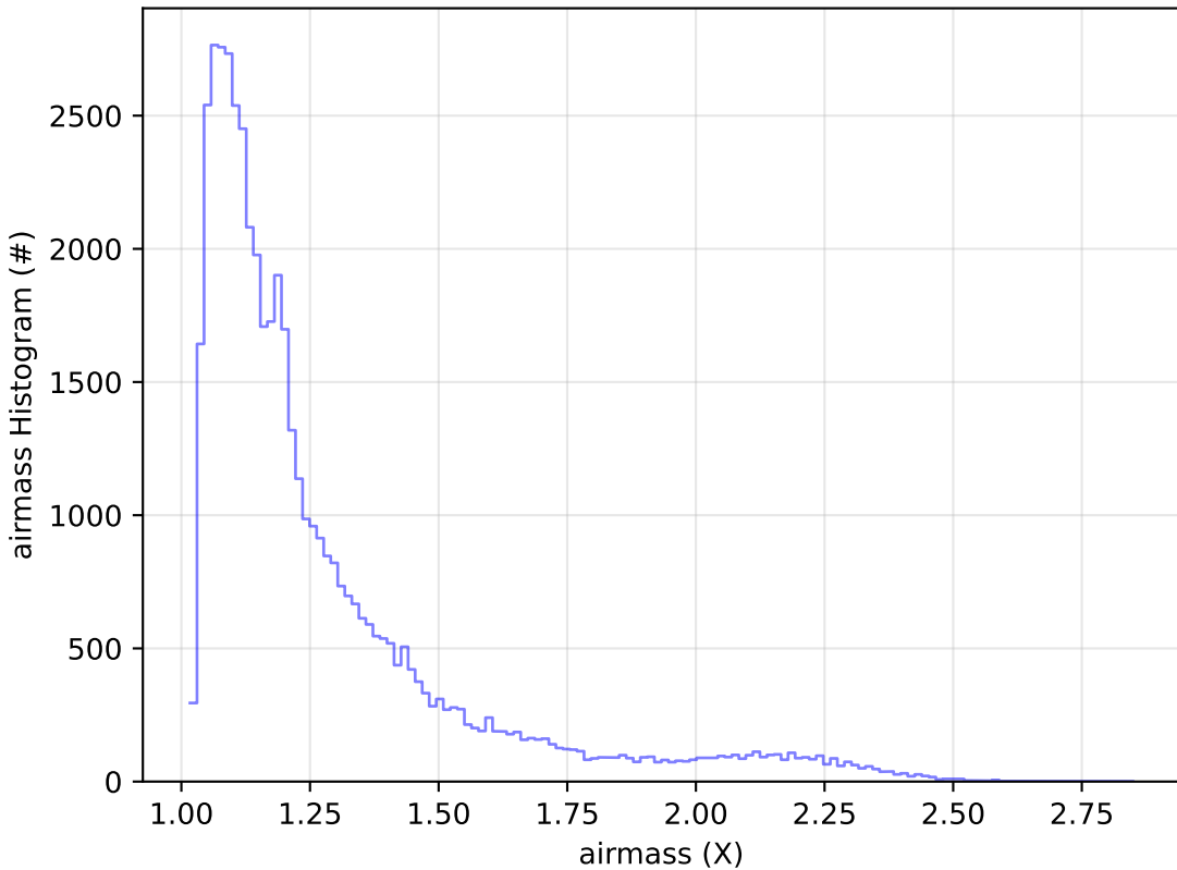
too_5_4v3.4_10yrs Yr 1 r band: airmass Histogram
