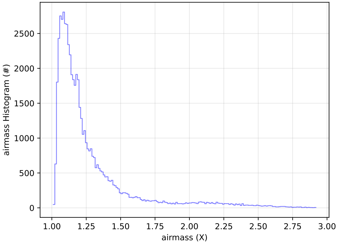
too_5_4v3.4_10yrs Yr 1 i band: airmass Histogram
