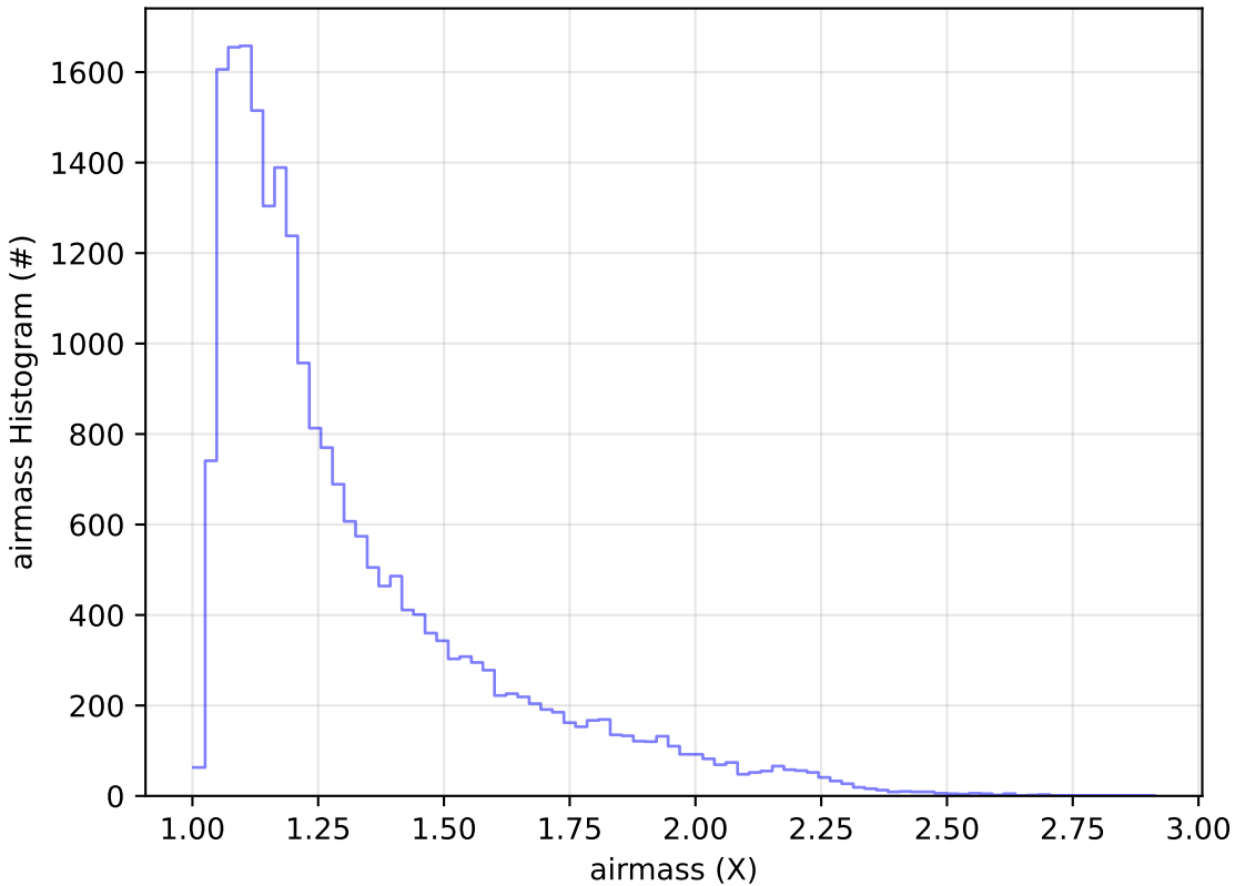
too_5_4v3.4_10yrs Yr 1 g band: airmass Histogram
