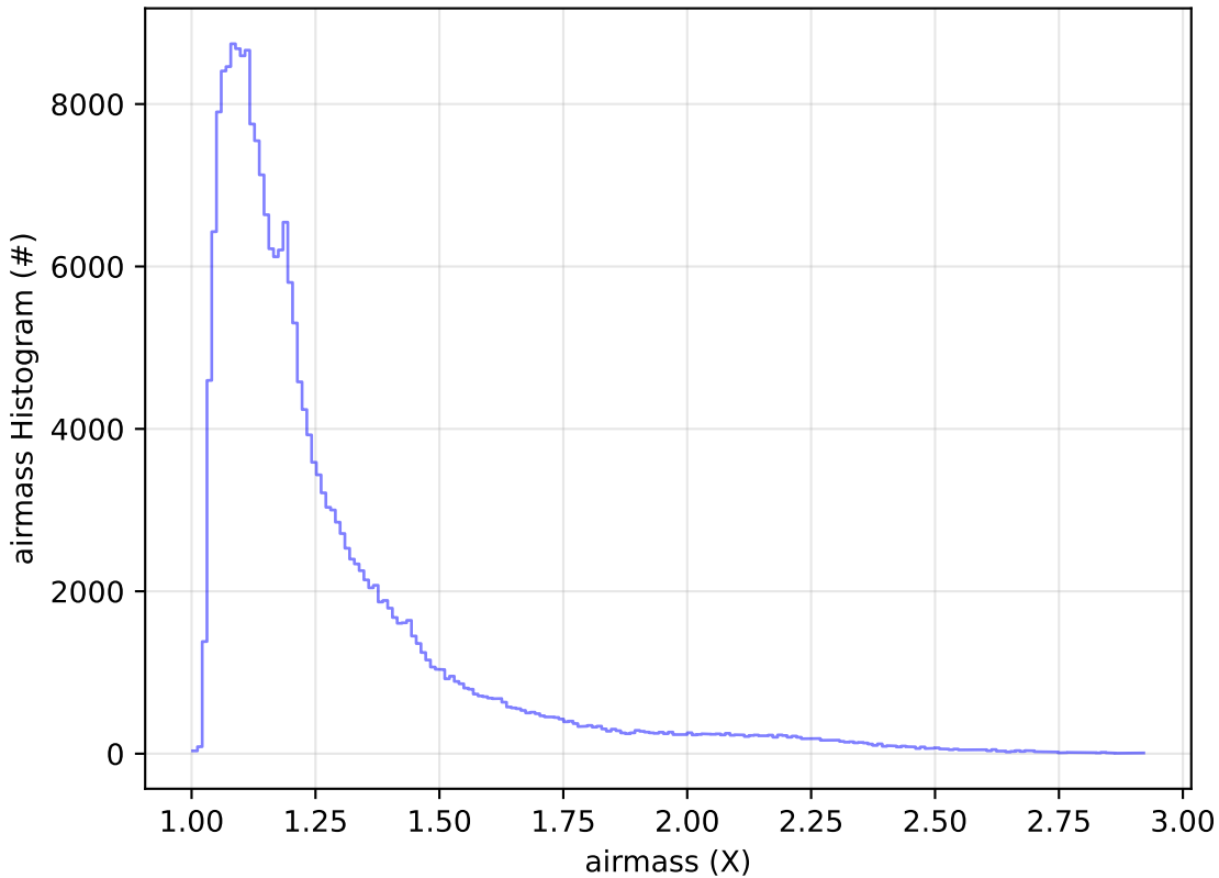
too_5_4v3.4_10yrs Yr 1 all bands: airmass Histogram
