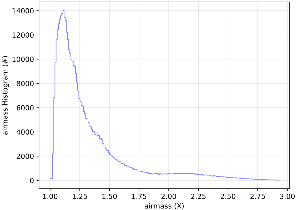
too_5_4v3.4_10yrs WFD z band: airmass Histogram
