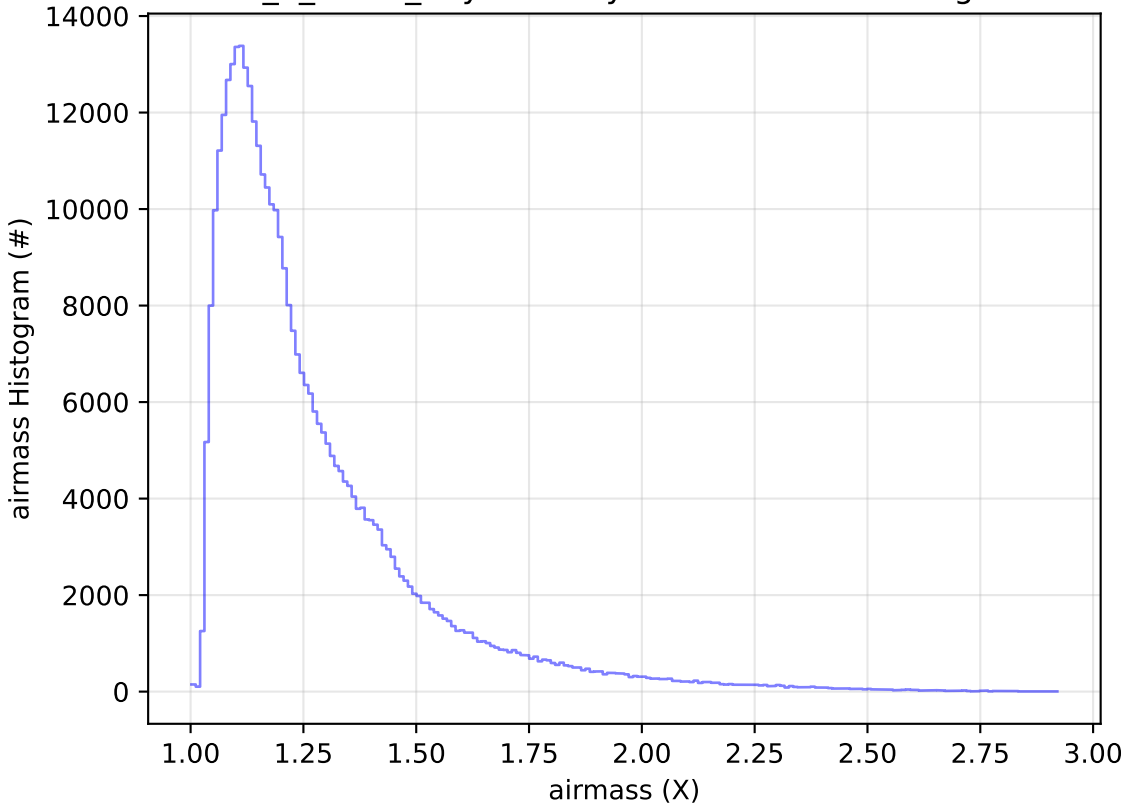
too_5_4v3.4_10yrs WFD y band: airmass Histogram
