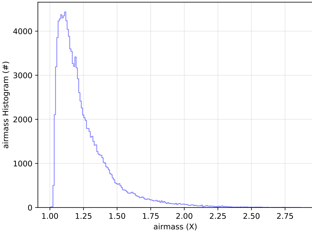
too_5_4v3.4_10yrs WFD u band: airmass Histogram
