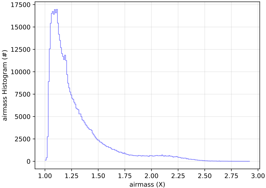
too_5_4v3.4_10yrs WFD r band: airmass Histogram
