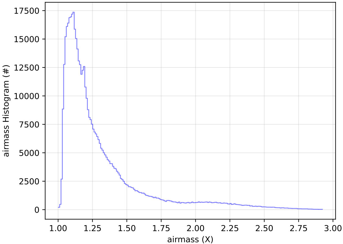
too_5_4v3.4_10yrs WFD i band: airmass Histogram
