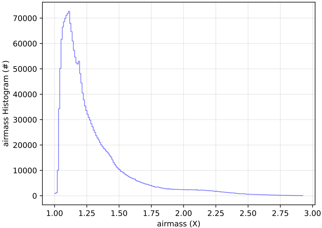
too_5_4v3.4_10yrs WFD all bands: airmass Histogram
