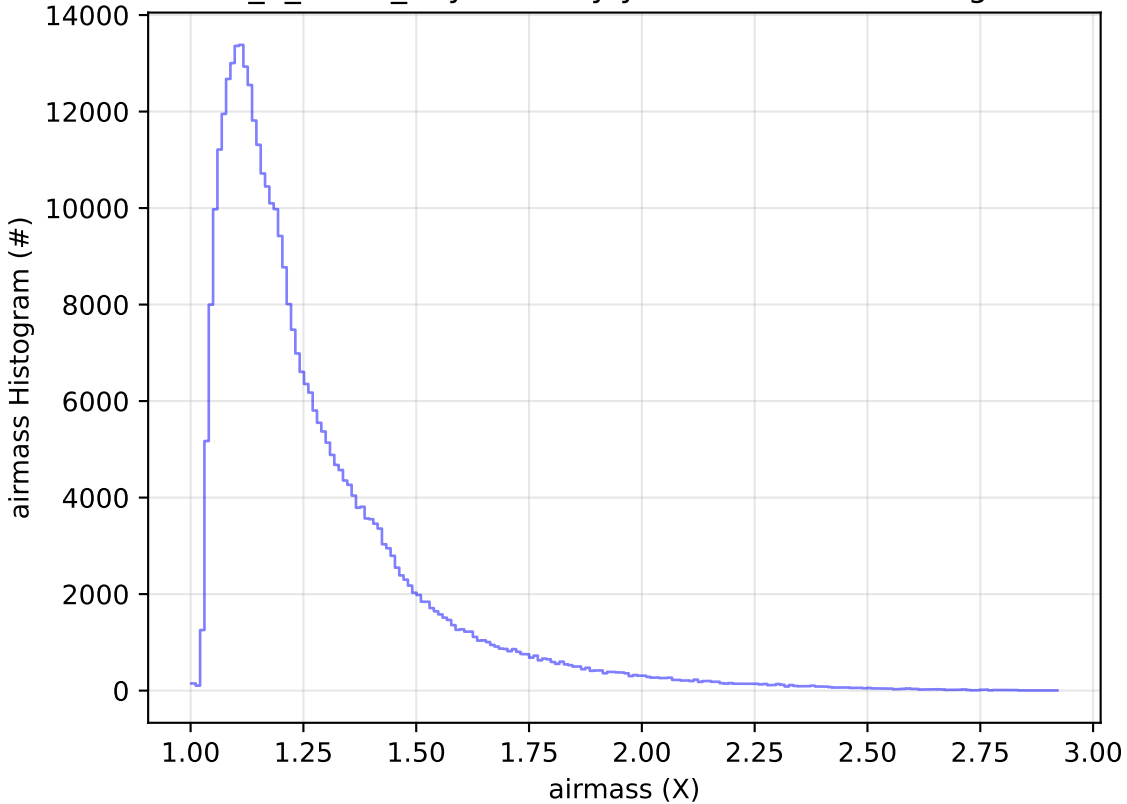
too_5_4v3.4_10yrs All sky y band: airmass Histogram
