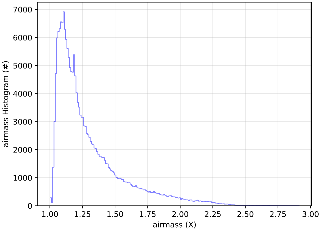
too_5_4v3.4_10yrs All sky g band: airmass Histogram
