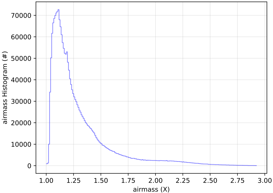
too_5_4v3.4_10yrs All sky all bands: airmass Histogram
