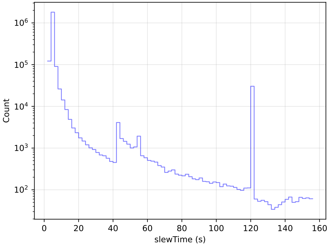
too_5_4v3.4_10yrs All visits: Slew Time Histogram
