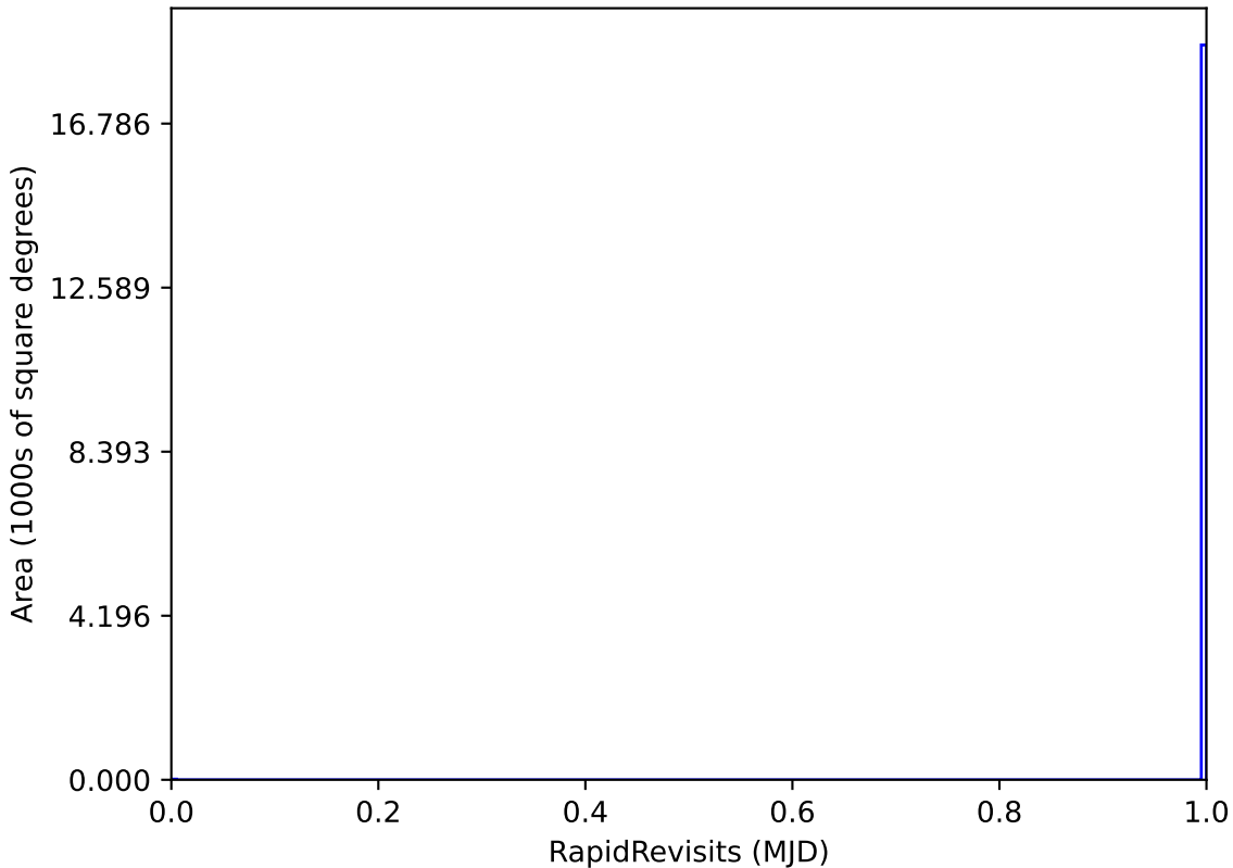
too_5_4v3.4_10yrs WFD: RapidRevisits
