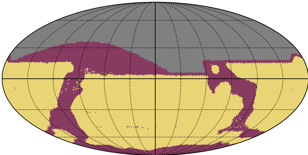
too_5_4v3.4_10yrs All sky: RapidRevisits
