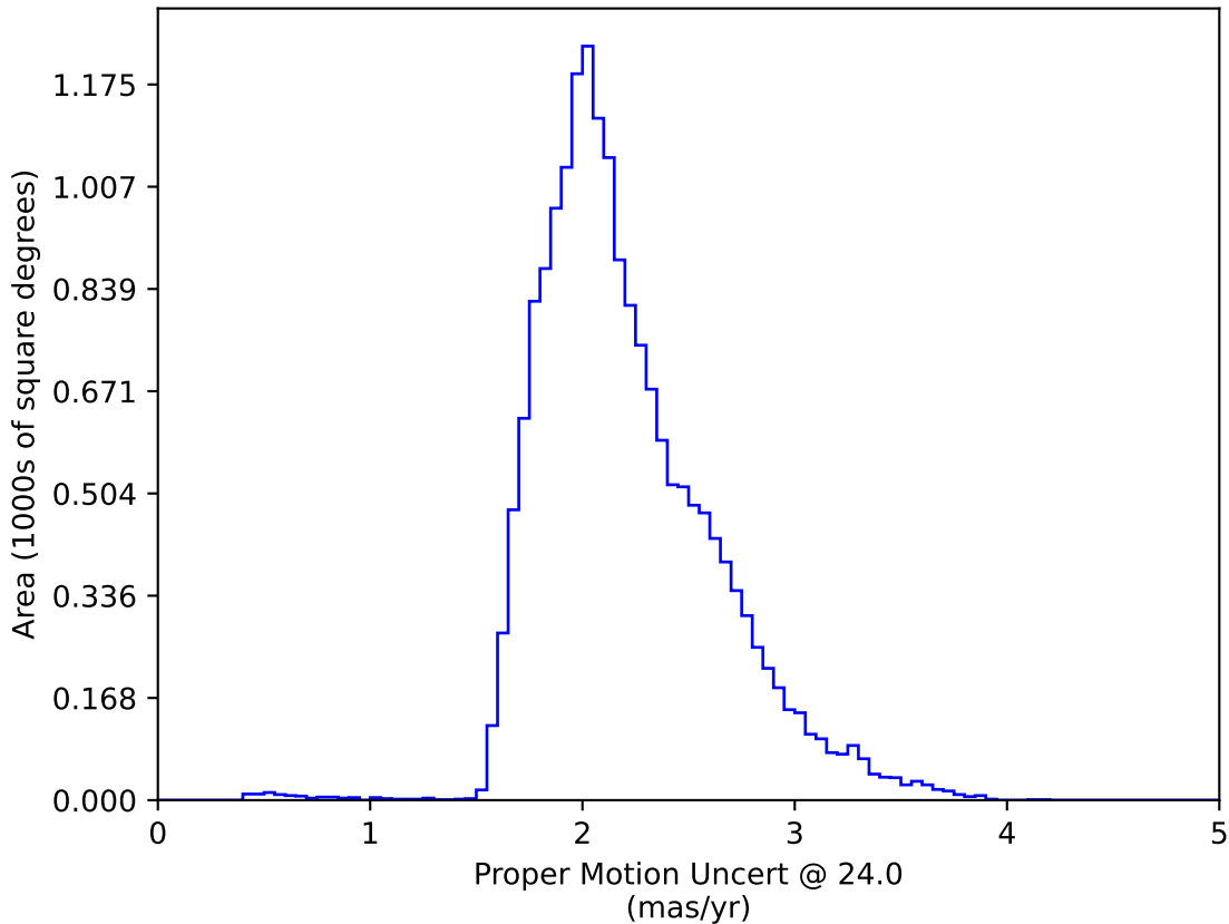
too_5_4v3.4_10yrs WFD: Proper Motion Uncert @ 24.0
