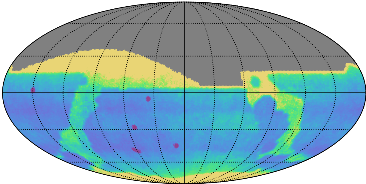
too_5_4v3.4_10yrs All sky: Proper Motion Uncert @ 24.0
