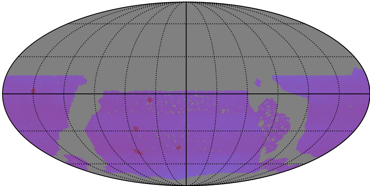
too_5_4v3.4_10yrs WFD: Proper Motion Uncert @ 20.5
