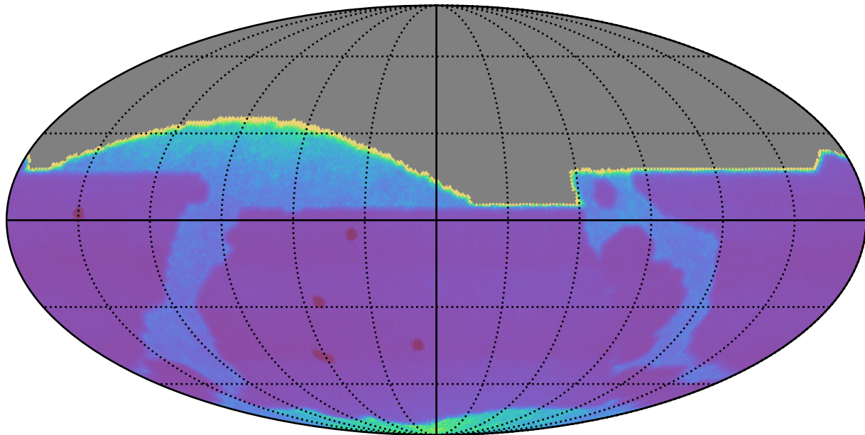
too_5_4v3.4_10yrs All sky: Proper Motion Uncert @ 20.5
