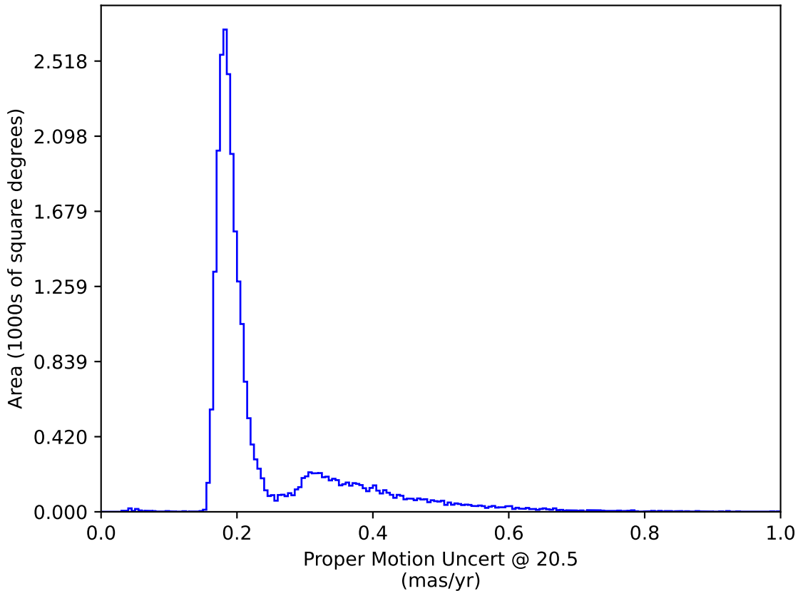
too_5_4v3.4_10yrs All sky: Proper Motion Uncert @ 20.5
